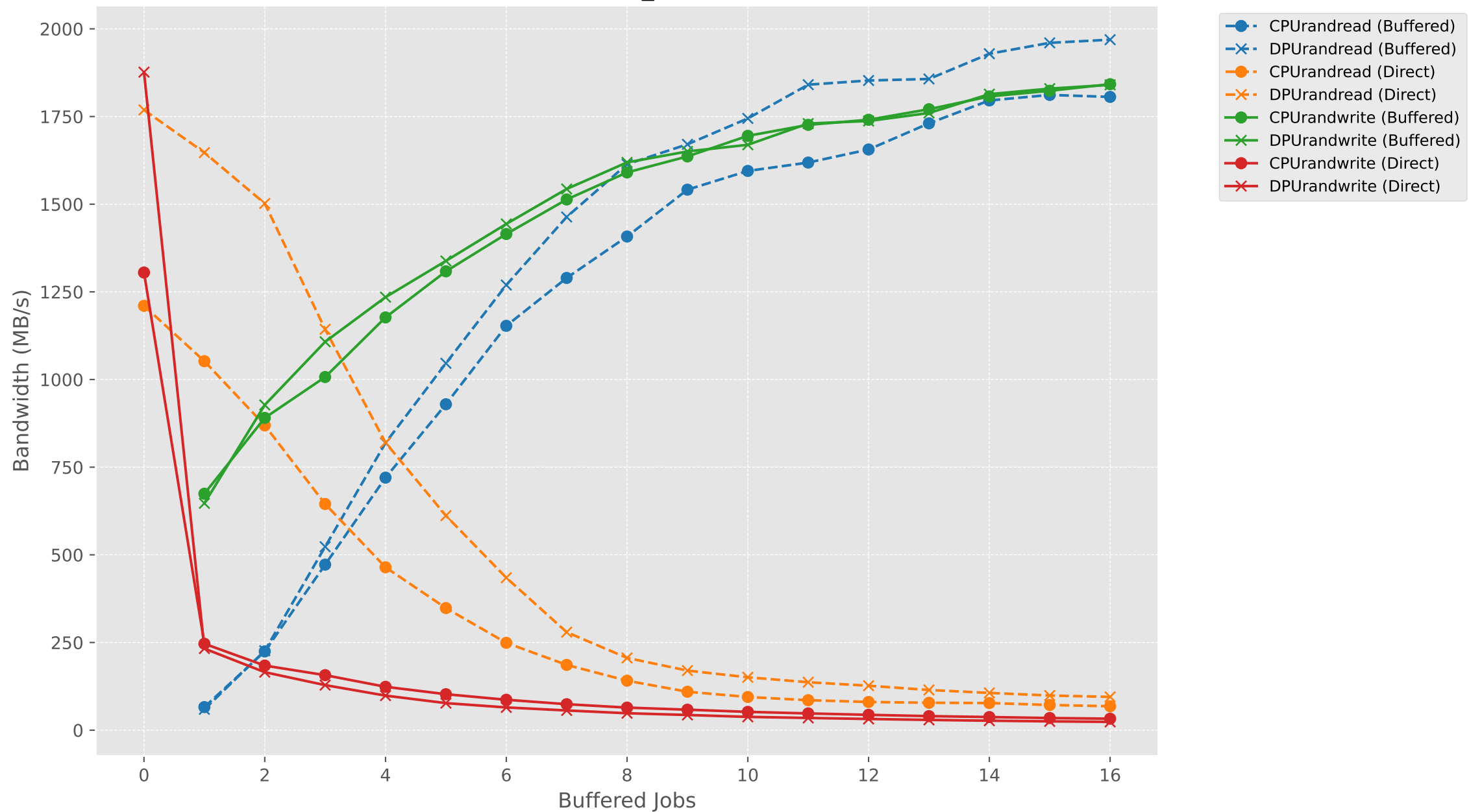
Bandwidth vs Buffered Jobs (direct1_bufferedN) - RAND (CPU vs DPU)
